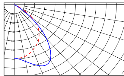
LBGT300282-56SS 2x28wT5 Semi Specular Test Report LSA9171.
