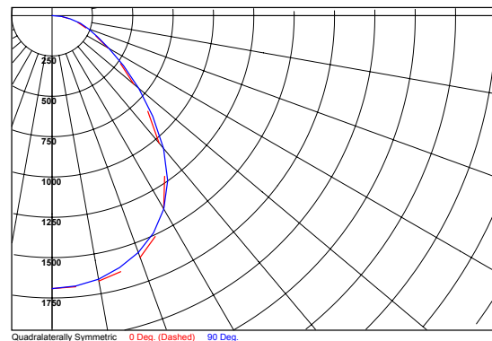
GEGRID300362Y12 2x36w T8 YP12 Lens Test Report AS1040
