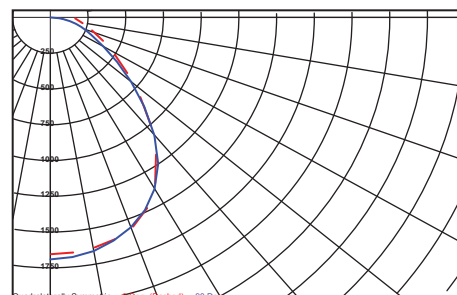
PLAS300362Y12 2x36w T8 Y12 Lens Test Report AS1041
