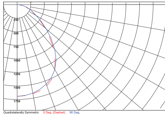
PLAS300362Y12 2x36w T8 YP12 Lens Test Report AS1041
