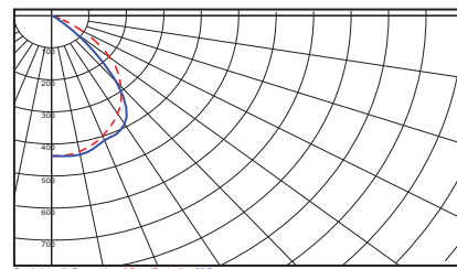
DIR600141 1x14w T5 Directlight Test Report LL11372
